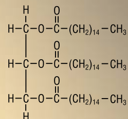
(E) glyceryltripalmitate
