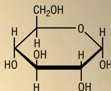
(B) glucose
